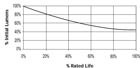
Lumen Maintenance
